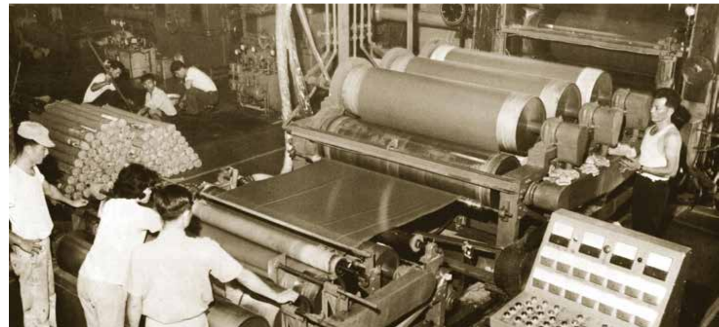
— The first adhesive tape machine of Nan Ya Plastics Corporation
